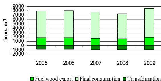
Fig.4. Fuel wood use in Latvia.
