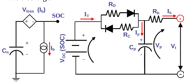
Figure .1. Run-time Battery dynamic Model [4, 6]
