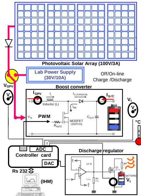
Figure .3. Photovoltaic system Testbench
