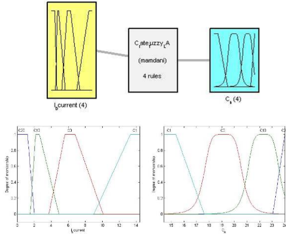
Figure .2. Membership function of input ( I_b ) and the output ( C_n )
