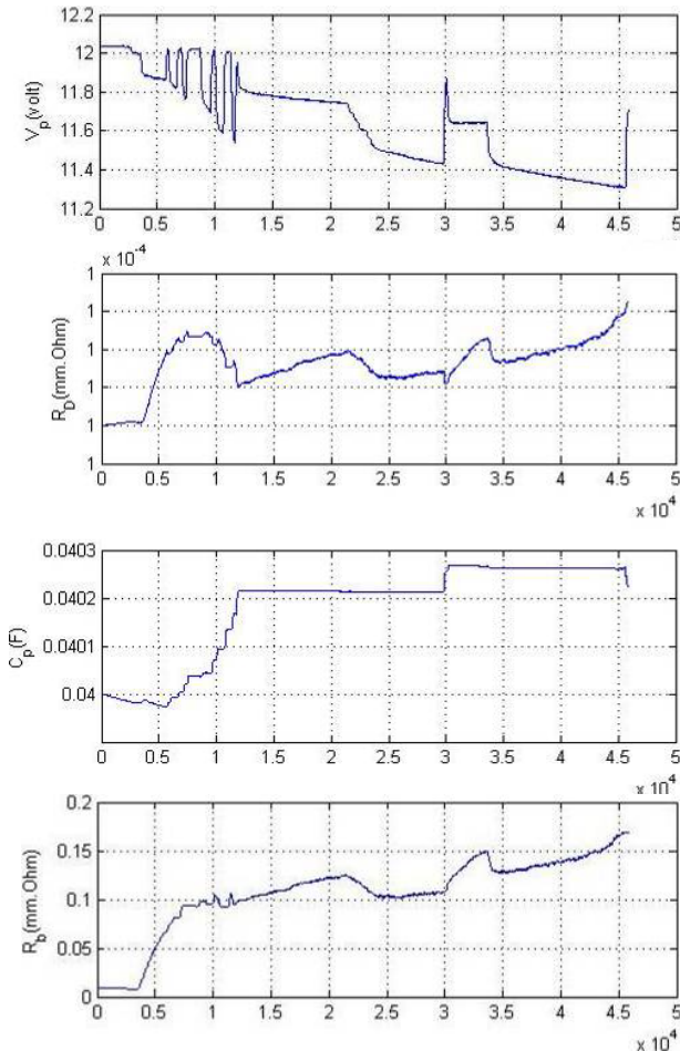
Figure .6. The estimated parameters
