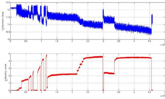
Figure .5. Evolution of the measurements ( I_b , V_t ) in discharge phase
