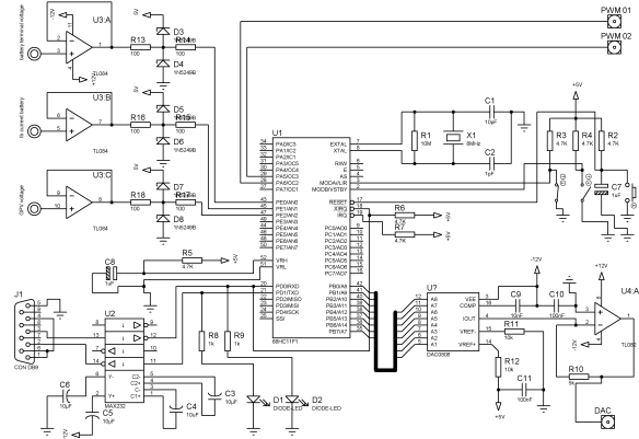
Figure .4. Testbench controller card
