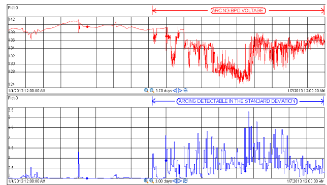
Figure 1. Standard deviation calculation and comparison for detecting erratic BPD voltages: BPD voltage (top) and standard deviation (bottom)
