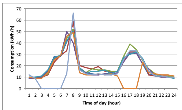
Figure 3. Hourly consumption as a function of time of day, during seven consecutive days for an agricultural customer
