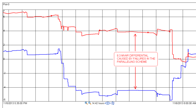
Figure 2. Transformers reactive power comparison for detecting correct paralleling
