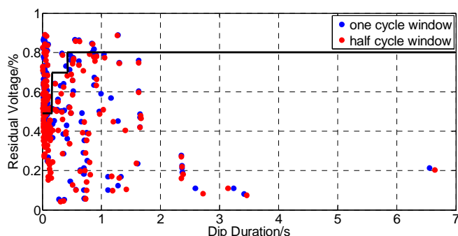
Fig. 15. Dip profile with SEMI F47-curve (longest event)
