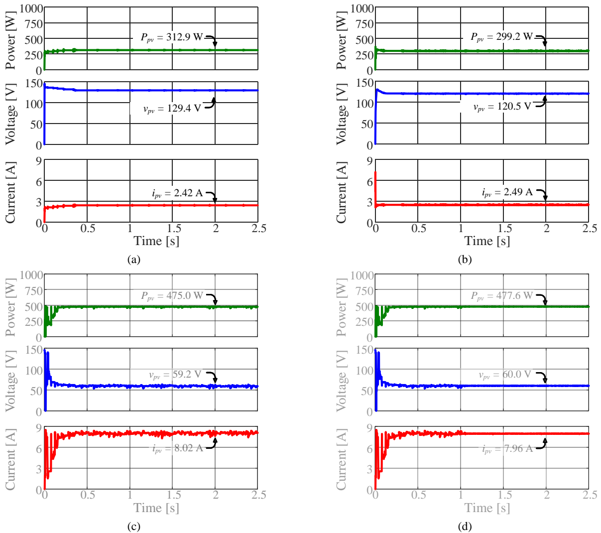
Fig. 9. Simulation results of MPPT techniques performance for case 2 (with partial shading): (a) P&O algorithm, (b) Beta Method, (c) GWO algorithm, (d) GWO-Beta algorithm. ( P_{pv} : 250W/div; v_{pv} : 50V/div; i_{pv} : 3A/div; time 0.5s/div).
