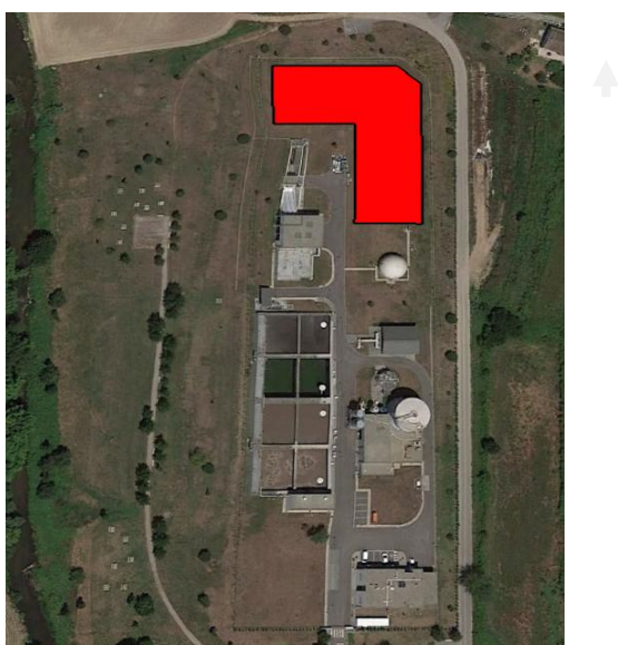
Fig. 3. Aerial view of the WWTP at Paço de Sousa and available area for solar plant installation (adapted from Google Earth 2021©).
