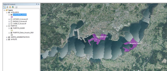
Fig. 7. Capture of the GIS project with the location of shipyards
