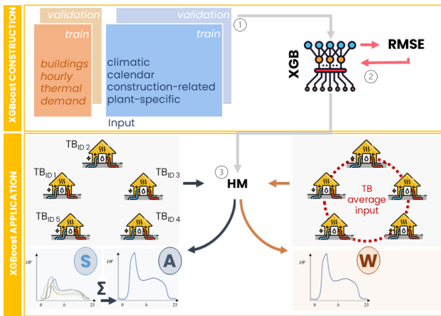
Fig. 1. Model's architecture
