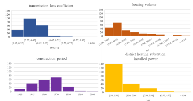
Fig. 2. Buildings' characteristics
