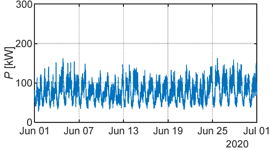
Fig.3. Transformer load profile for June
