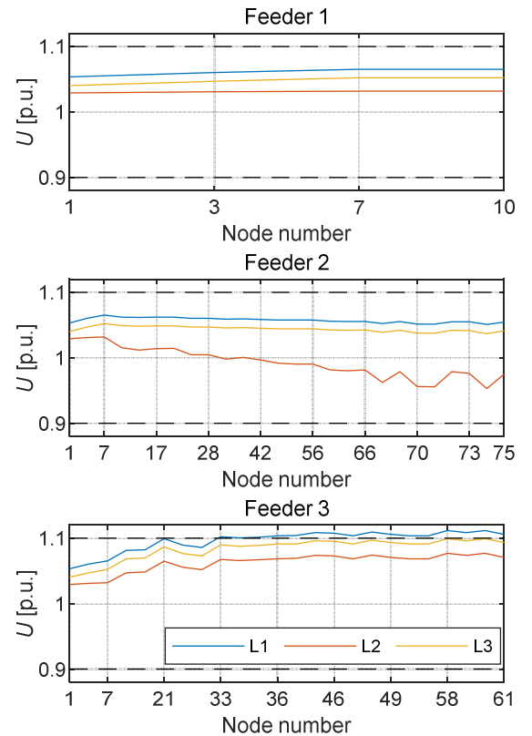
Fig.10. Voltage profile in Feeders 1, 2 and 3 for PV system integration into Feeder 3 according to approach II
