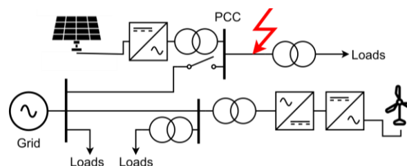
Fig. 1: Microgrid scheme.
