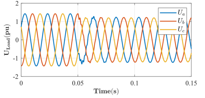
Fig. 4: Phase-to-neutral fault voltages and phase-to-phase load voltages when fault conditions imposed in the MB at t=0.05 s.
