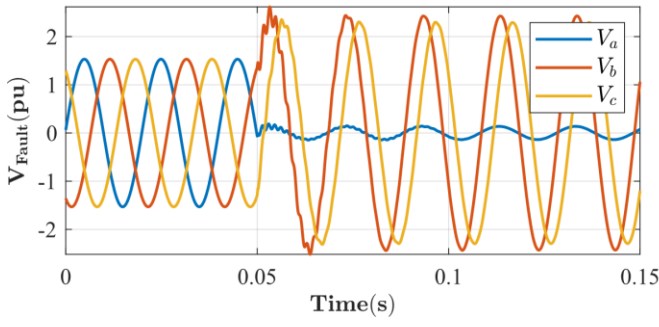
Fig. 4: Phase-to-neutral fault voltages and phase-to-phase load voltages when fault conditions imposed in the MB at t=0.05 s.
