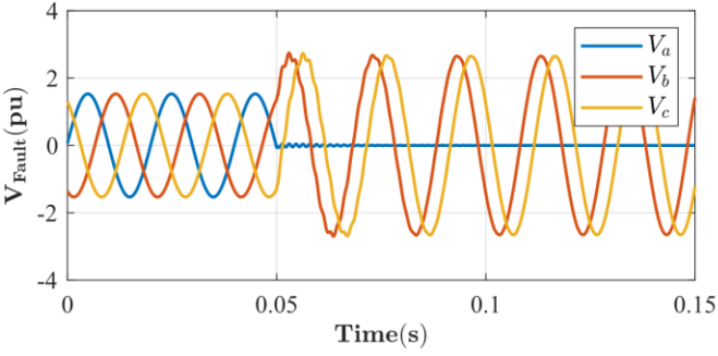
Fig. 5: Phase-to-neutral fault voltages and phase-to-phase load voltages when fault conditions imposed in the fault point at t=0.05 s.
