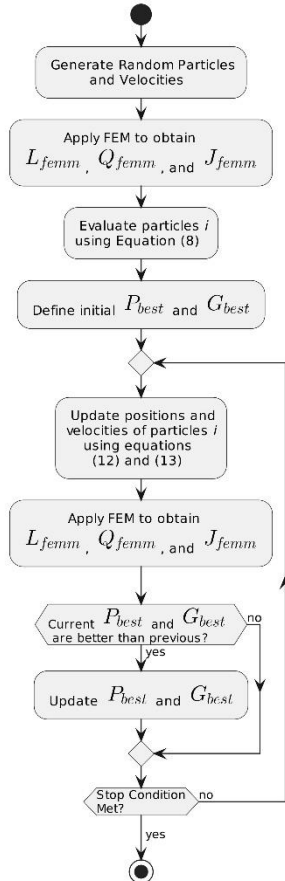
Fig. 2. Flowchart of the proposed optimization model.
