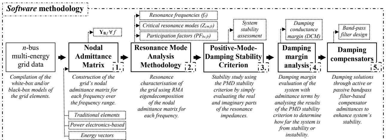
Fig. 1. Flowchart of the software methodology.
