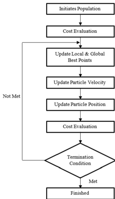
Fig. 3. Flow diagram of PSO
