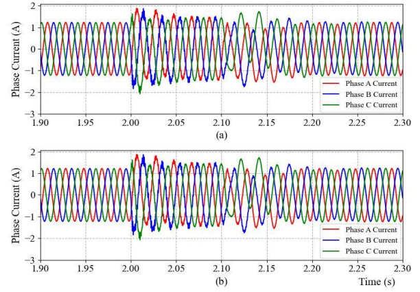
Fig. 6 Transient waveforms of the current before and after the optimization: (a) phase current before optimization (b) phase current after optimization
