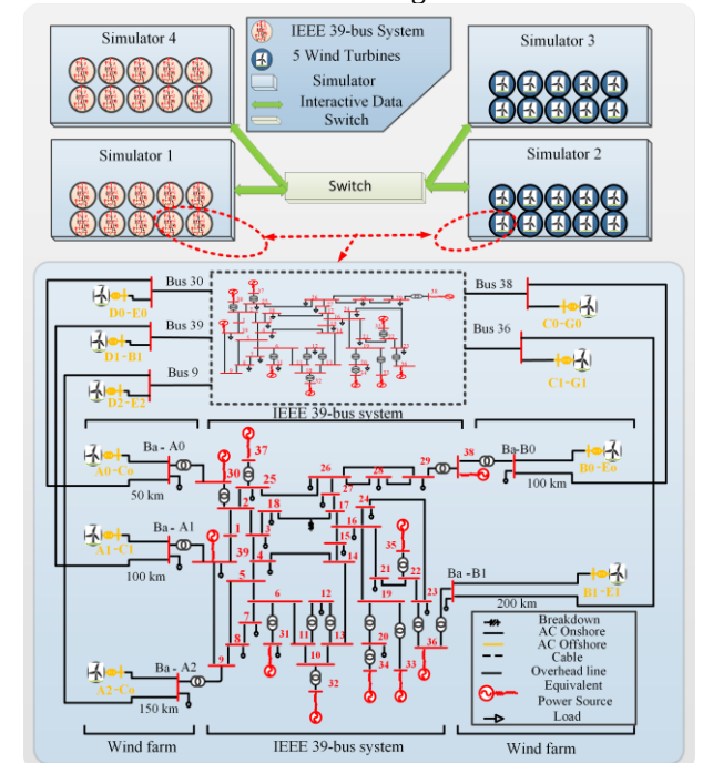
Fig. 4 Partition and the communication of the case study
