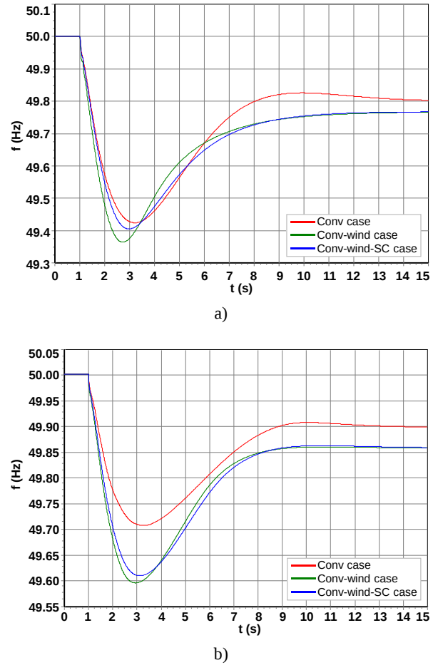
Fig. 4. System frequency time evolution for a sudden disconnection of the Diesel 9 generator unit of Punta Grande power plant for conv case, conv-wind case and conv-wind-SC case ( H_{SC} = 2 \text{ MWs/MVA} ): a) off-peak demand state; b) peak demand state.
