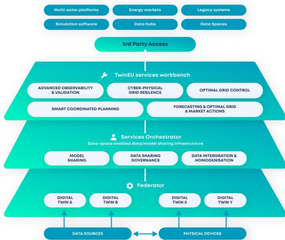
Fig. 2. TwinEU architecture ([3])
