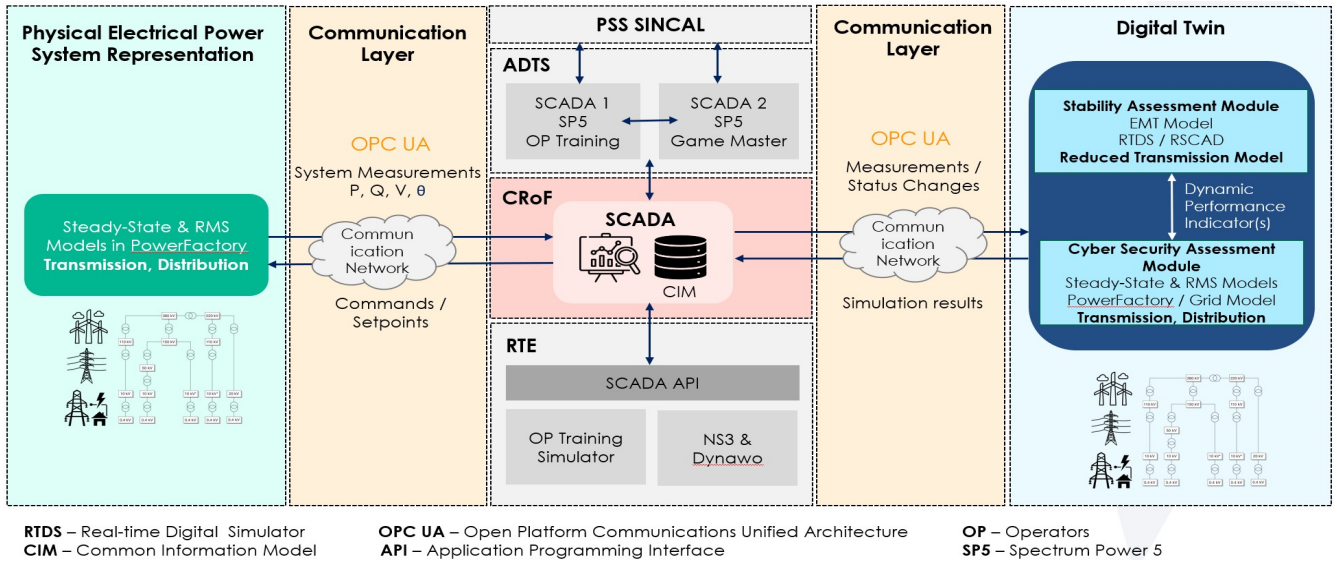
Fig. 4. The Dutch integrated digital twin architecture ([4])
