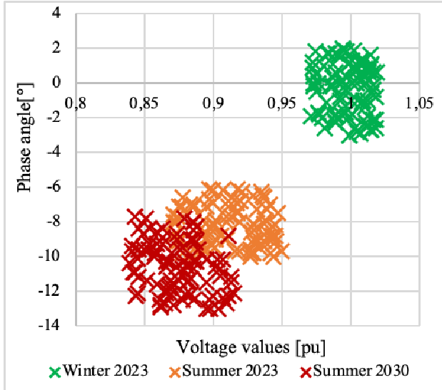
Fig.3. Voltage values on the 50Hertz grid
