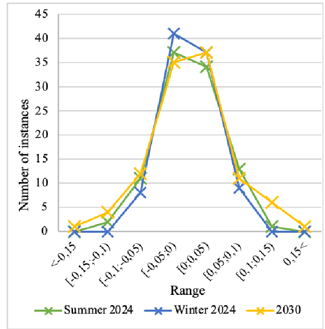
Fig.6. Distribution of ROCOF values on the Balearic Islands grid
