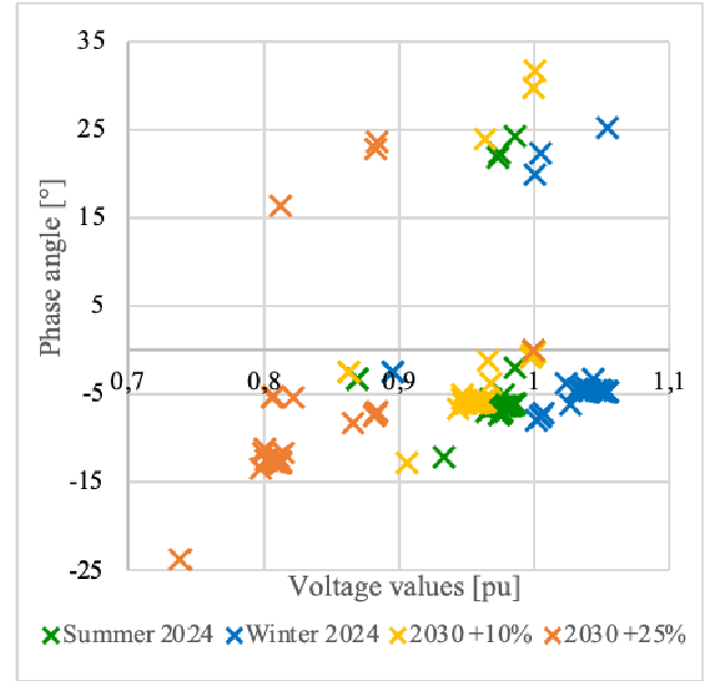
Fig.4. Voltage values on the Balearic system
