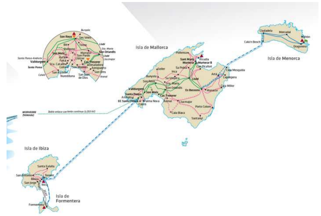
Fig.2. Transmission system of the Balearic Islands [12]
