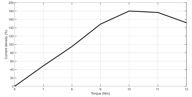
Fig.4. Current density performance as a function of the torque.
