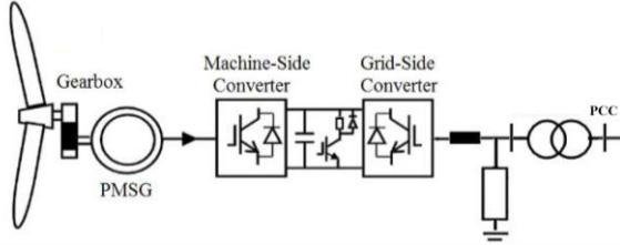
Fig. 3. Scheme of the wind turbine under study.
