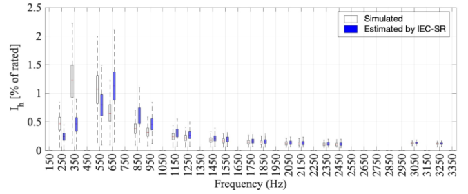
Fig. 8. Comparison between the measured emission harmonic currents at PCC obtained by the SM (Simulated in the legend) and those obtained applying IEC-SR (Estimated by IEC-SR in the legend).
