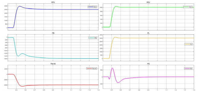
Fig.5. Instantaneous power of each element of the nZEH in Scenario 2.
