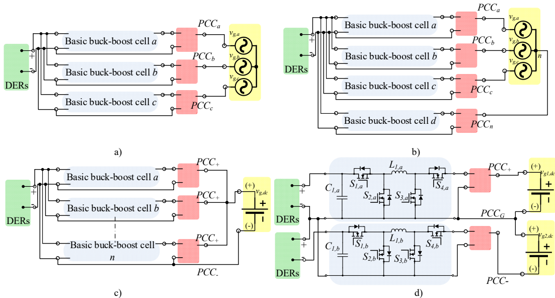
Fig. 2. Proposed configurations in [10]: a) three cells for dc-ac three-phase three-wire. b) four cells for dc-ac three-phase four-wire. c) n cells for dc-dc (interleaved) and d) two cells for dc-dc bipolar.
