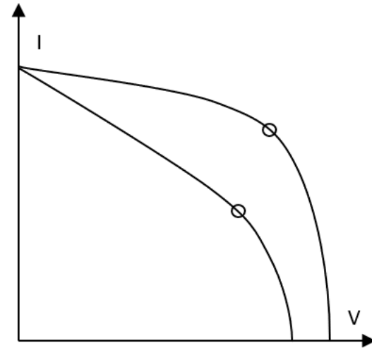
Fig. 3. Original PV and PV with parallel resistor. Maximum power points in circles
