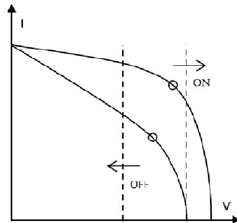
Fig. 6. Hysteresis control on PV characteristic.
