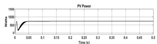
Fig. 10. Behaviour of a MPPT in the normal case.
