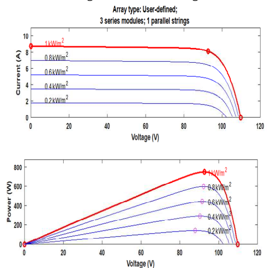
Fig. 9(a-b). Simulation of 3 panels in series, one string in parallel, normal case: Voltage/current and Voltage/Power
