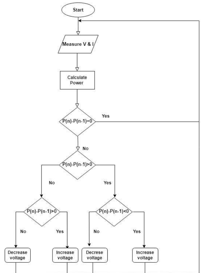
Fig.8. MPPT P&O Algorithm
