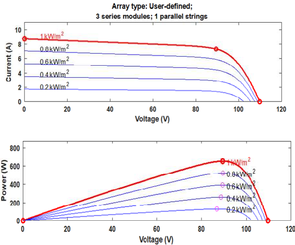
Fig. 11(a-b). Simulation of 3 panels in series, one string in parallel, 30 ohm in parallel: Voltage/current and Voltage/Power
