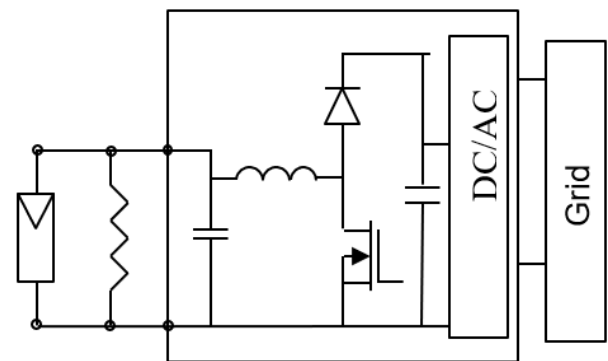
Fig. 4: Basic circuit
