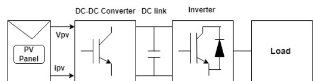
Fig.1.Solar PV system
