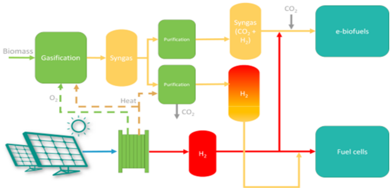
Fig. 1. Integration of electrolysis and biomass gasification concept in AIHRE project
