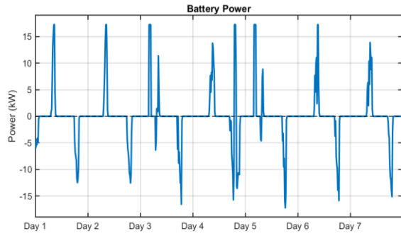
Fig. 8. Battery power profile over time in Scenario I.
