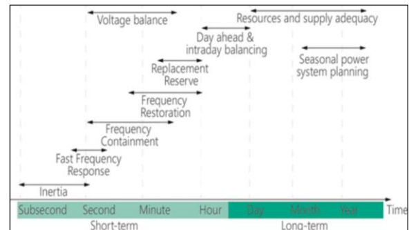
Fig. 14. Time horizon of the flexibility services provided by hydroelectric power plants [8]
