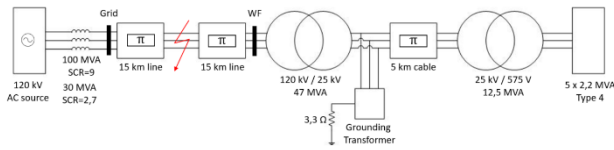
Fig.1. Network model in Matlab/Simulink
