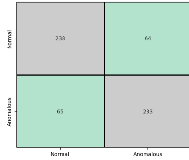
Fig.5. Confusion matrix for data error detection of the High-Speed Shaft downwind bearing radial sensor.
