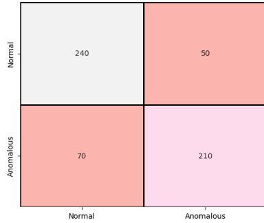
Fig.4. Confusion matrix for data error detection of the High-Speed Shaft Upwind Bearing Radial sensor.
