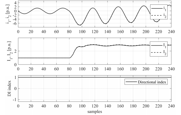
Fig. 11. External fault: current waveforms, RMS indicators, and directional index
