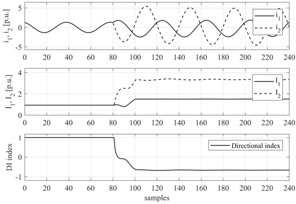
Fig. 5. 50% Inter-turn fault case: current waveforms, RMS indicators, and directional index.
