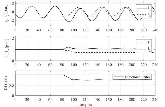
Fig. 7. 10% Interturn fault case for PT positioned between the active and passive networks
