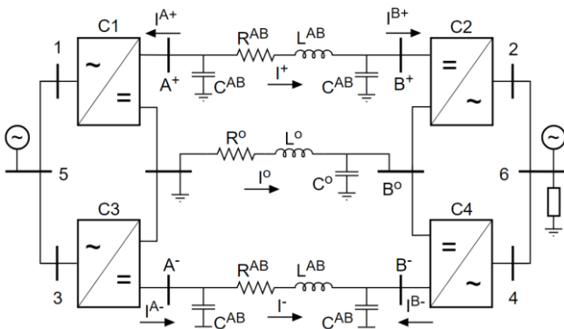
Fig. 1. Bipolar HVDC link model with metallic return.
