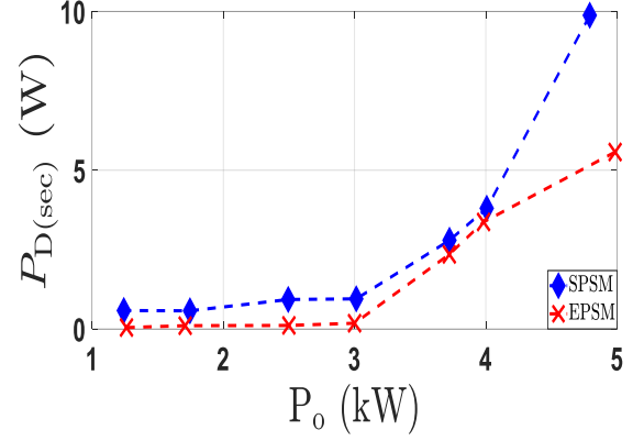
Fig. 10. Secondary-side S_5 diode losses for SPSM and EPSM under different loading conditions
