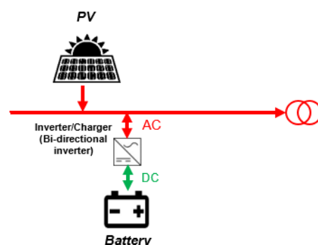
Fig.1. PV-battery power generating system.
