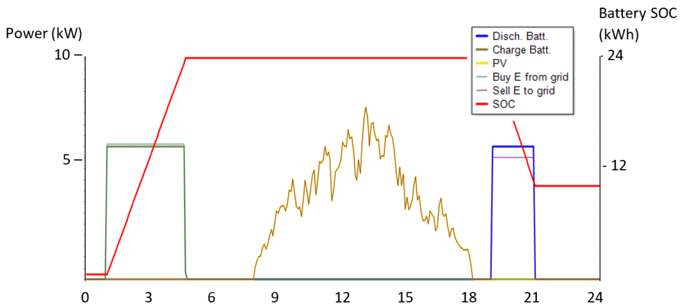
Fig. 7. Simulation of the optimal arbitrage strategy obtained with two variables method [7].
