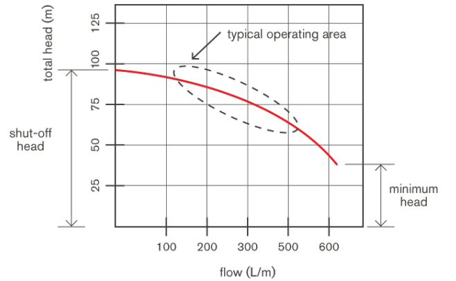
Fig. 6. Typical pump performance curve of total head versus flow rate.
