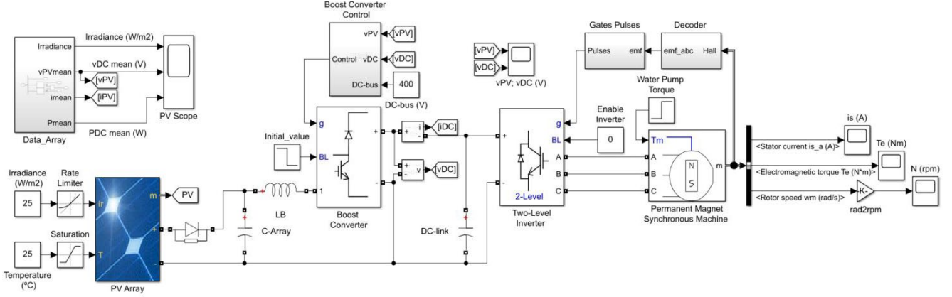
Fig. 9. Stand-alone photovoltaic water pumping system model. The model has been developed in Matlab/Simulink software. Temperature (°C) and irradiance (W/m²) have been considered as input parameters to the system [7].
