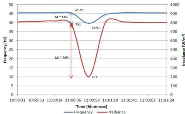
Fig. 2. Variation in the irradiance and frequency of the water pump during the passage of a cloud in a stand-alone photovoltaic water pumping system.
