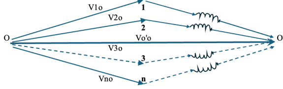
Fig.1: indicates the Millman's Theorem network
