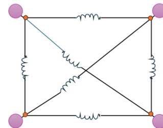
Fig. 6c equivalent circuit via Park's reduction formula
