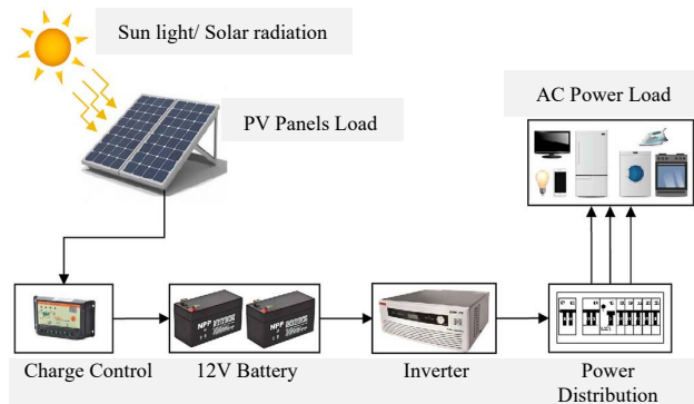
Figure 11: Power Conversion schematic in Solar system
