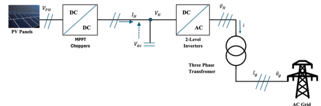
Fig.2 Solar system power generation schematic
