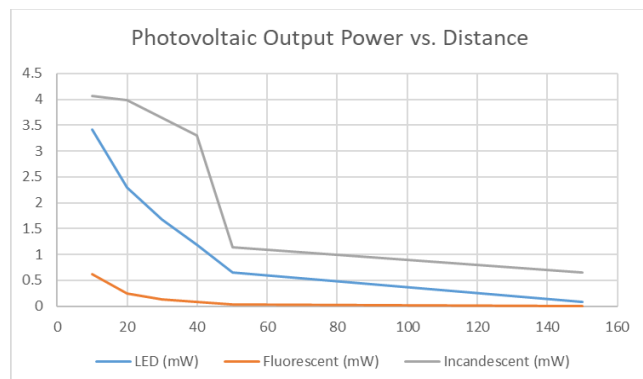
Fig. 6 The variation of the photovoltaic module output power as a function of the distance
