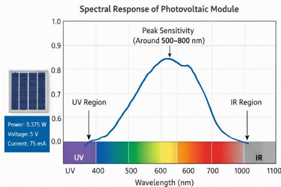
Fig. 4 Spectral Response of Photovoltaic Module
