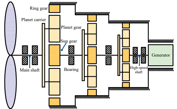
Fig.2. Modeling of the 15 MW integrated wind turbine drivetrain
