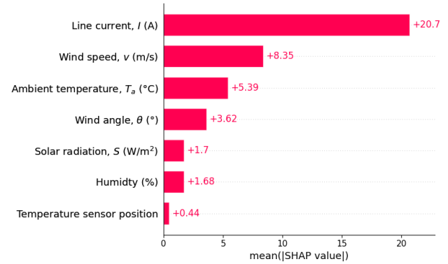
Fig. 4. Global feature importance based on mean absolute SHAP values.
