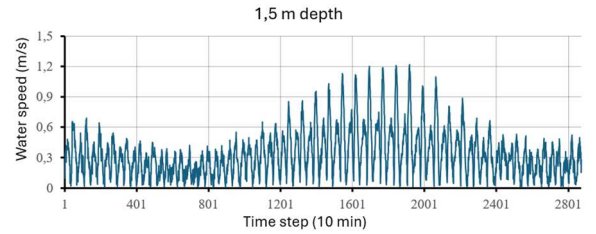
Fig.4. Time series of water velocity at 1.5 m depth recorded by ADCP at the deployment site over a complete spring–neap cycle (10 min sampling interval).
