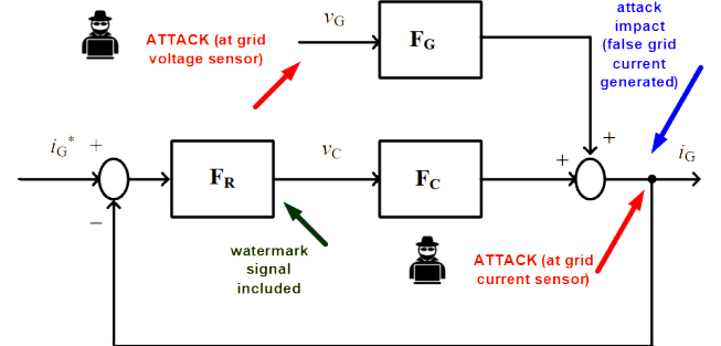
Fig. 2 Simplified block diagram of control system for grid-connected converter via LCL grid filter, indicating watermark injection points, potential attack locations, and attack detection points.
