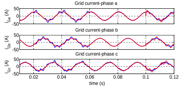
Fig. 6 Time responses of grid phase currents i_{Ga} , i_{Gb} , i_{Gc} for the system model without watermark signal (red) and real grid current responses with watermark and attack (blue)
