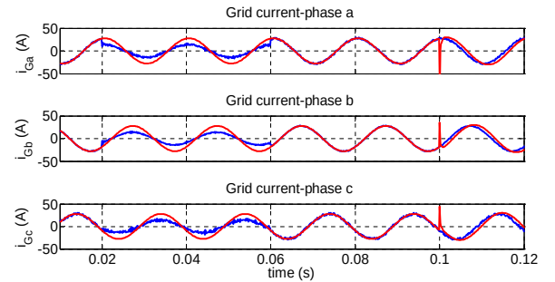
Fig.3. Time responses of grid phase currents i_{Ga} , i_{Gb} , i_{Gc} for system model without watermark signal (red) and grid current responses with watermark and attack (blue)
