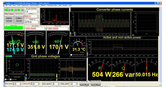
Fig. 8 Example of the dSPACE™ control panel layout
