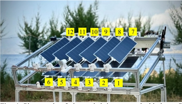
Fig. 1 Photograph of the scaled in power double-layer PV prototype.
