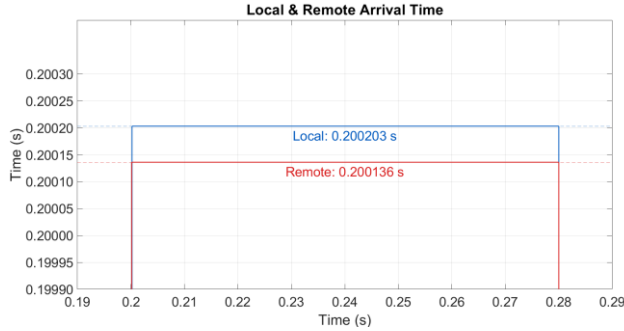
Fig. 7. Local and remote arrival time.
