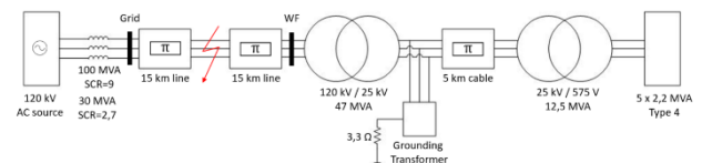
Fig. 2. Network model.
