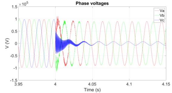
Fig. 3. Phase voltages.
