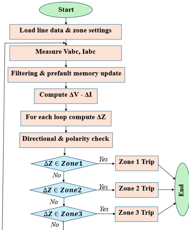
Fig. 1. IQ based distance protection flowchart.
