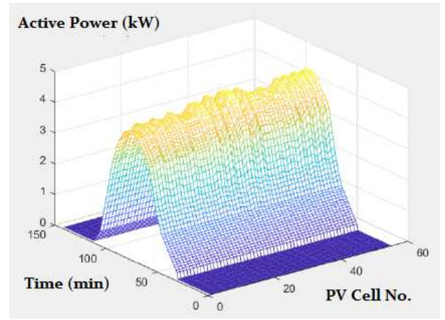
Fig 11. Active Power of the PV Cells
