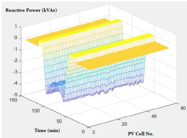
Fig 15. Reactive Power of the PV Cells
