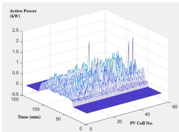
Fig 5. Active Power of the PV Cells
