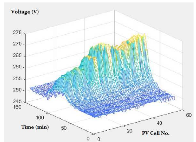
Fig 7. Voltage of the PV Cells
