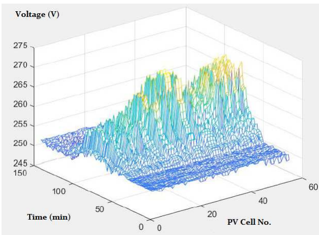
Fig 10. Voltage of the PV Cells
