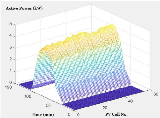
Fig 14. Active Power of the PV Cells
