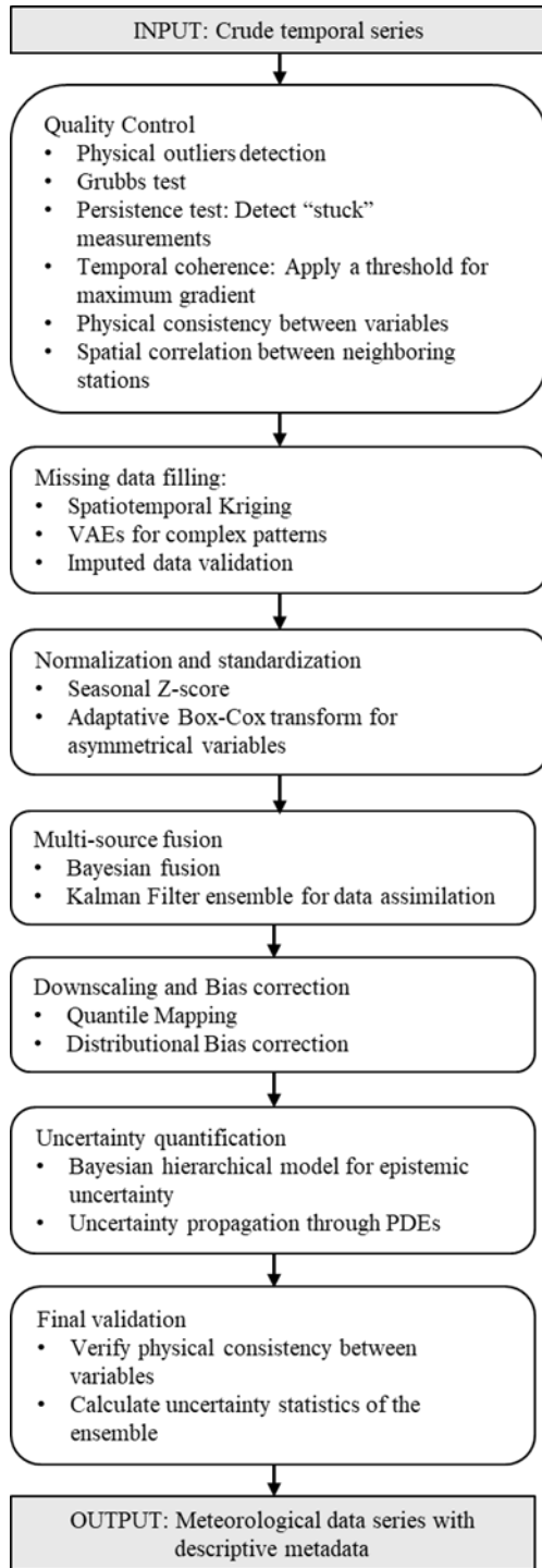
Fig. 2. Preprocessing of Meteorological Time Series pipeline
