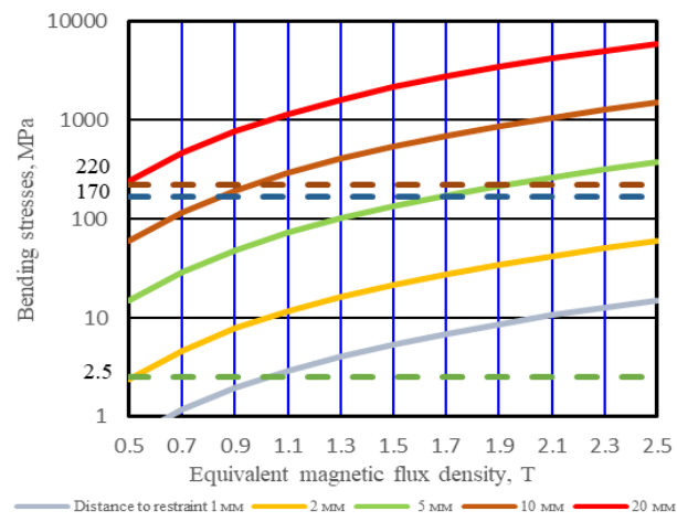
Fig. 2 Bending stresses in tangential restraint
