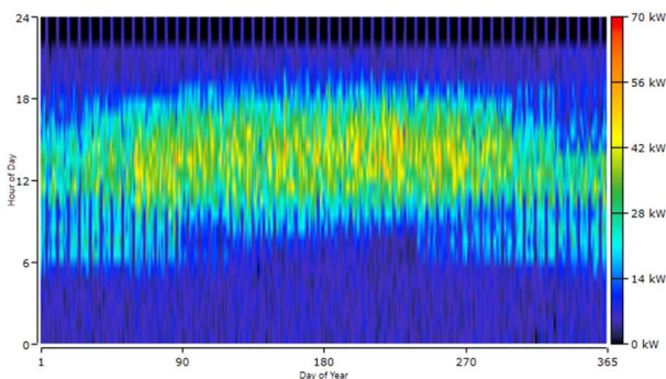
Fig. 1. Electrical demand.
