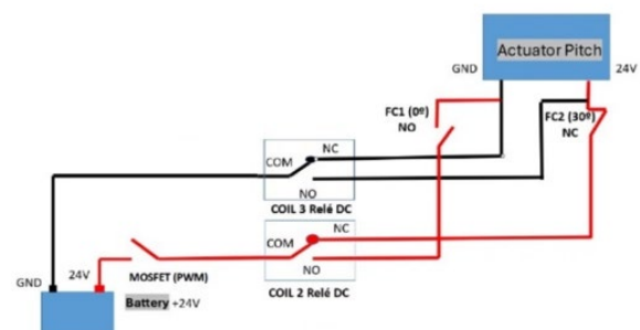
Fig. 4. Pitch control scheme
