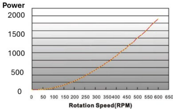
Fig. 1. Output power versus rotation speed
