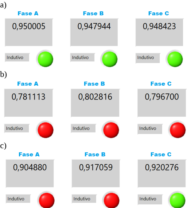
Fig. 11. Power Factor dynamics detected by the software: (a) Baseline operation; (b) Inductive load step; (c) Reactive power compensation.
