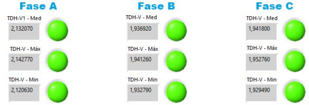
Fig. 12. Total Harmonic Distortion ( THD_V ) analysis.
