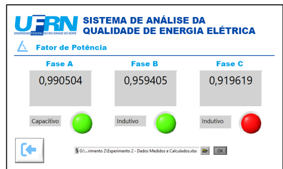
Fig. 6. Power Quality interface focusing on Power Factor analysis and compliance verification.
