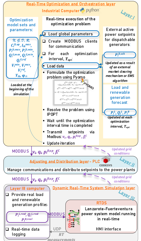
Fig. 1. RT optimization-based control architecture in RTOLab
