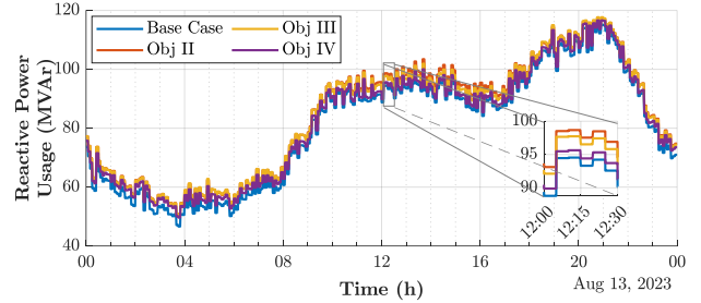
Fig. 5. Total reactive power utilization over the 24-hour period
