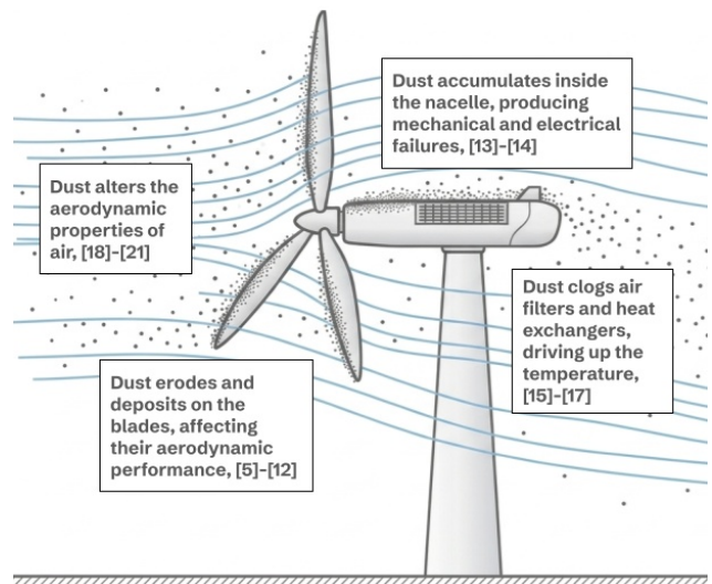
Figure 2. Graphical summary of the four main challenges faced by wind turbines operating in the presence of dust.
